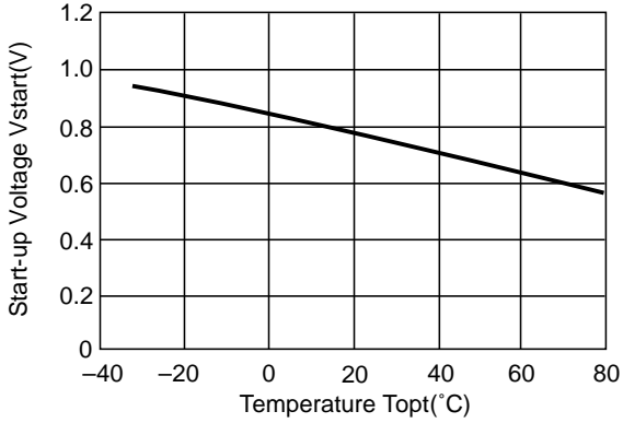
7) Start-up Voltage vs. Temperature
